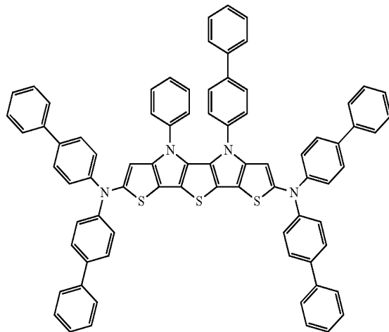
[Chemical Formula 48]
