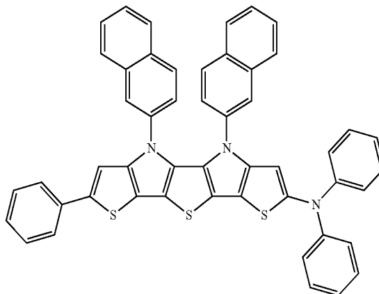
Chemical Formula 17
