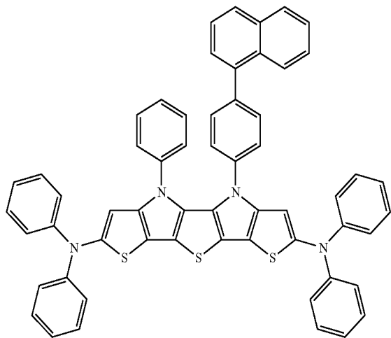
[Chemical Formula 25]
