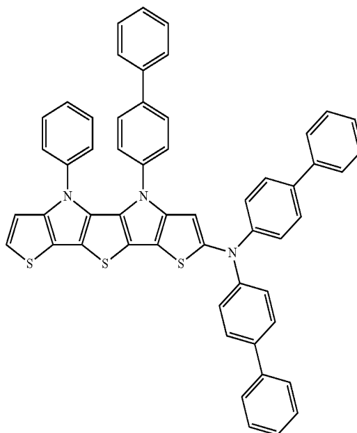
[Chemical Formula 32]
